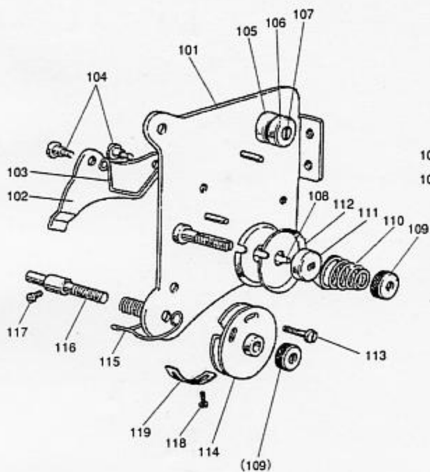
Fig.901 LU2-4400-B0B
