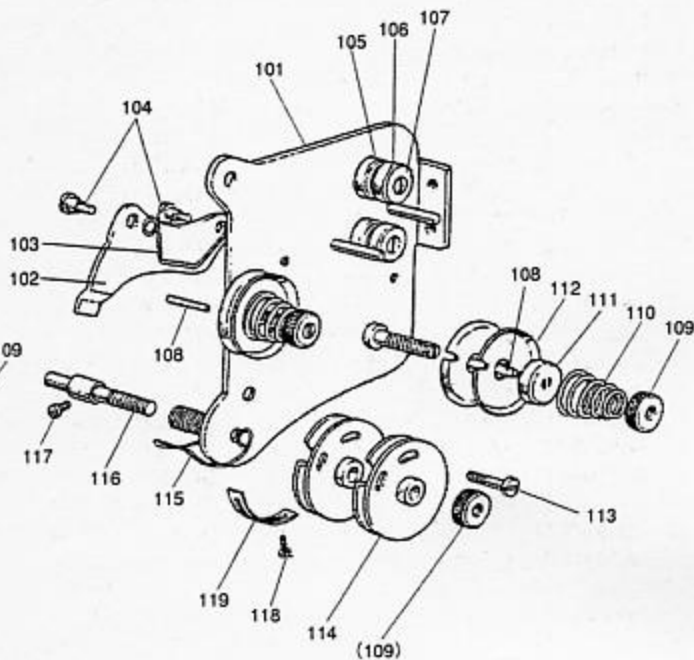
Fig.902 LU2-4420-B0B
