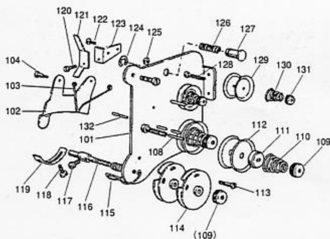
Fig.904 LU2-4430-B1T
